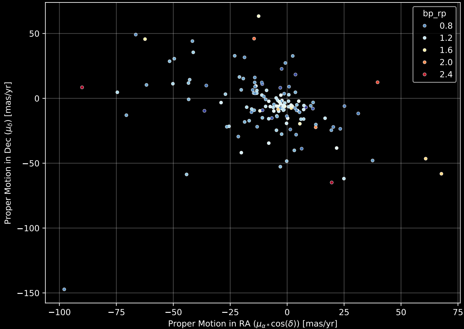
APOGEE DR17 Field: [042+43_MGA] Proper Motion Diagram (n= 142)
