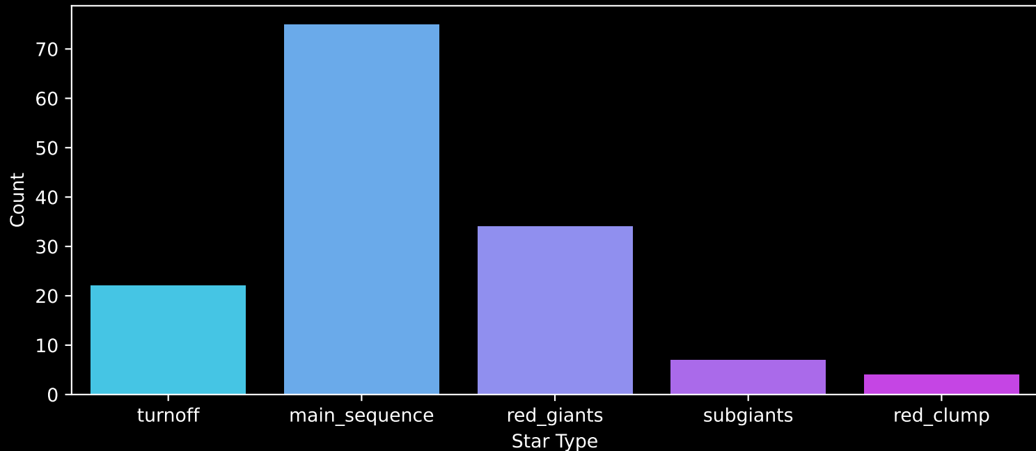
APOGEE DR17 Field: [042+43_MGA] Count plot of Star Type
