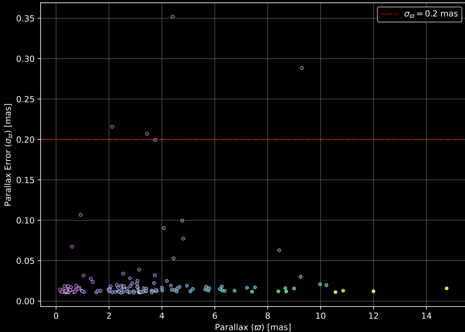
APOGEE DR17 Field: [042+43_MGA] Parallax Quality (n= 142)
