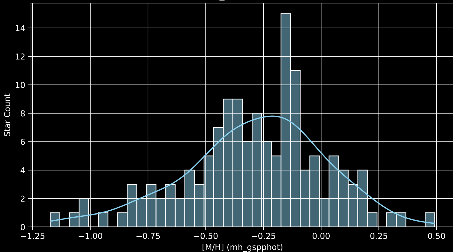
APOGEE DR17 Field: [042+43_MGA [M/H] (mh_gspphot) (n= 140)
