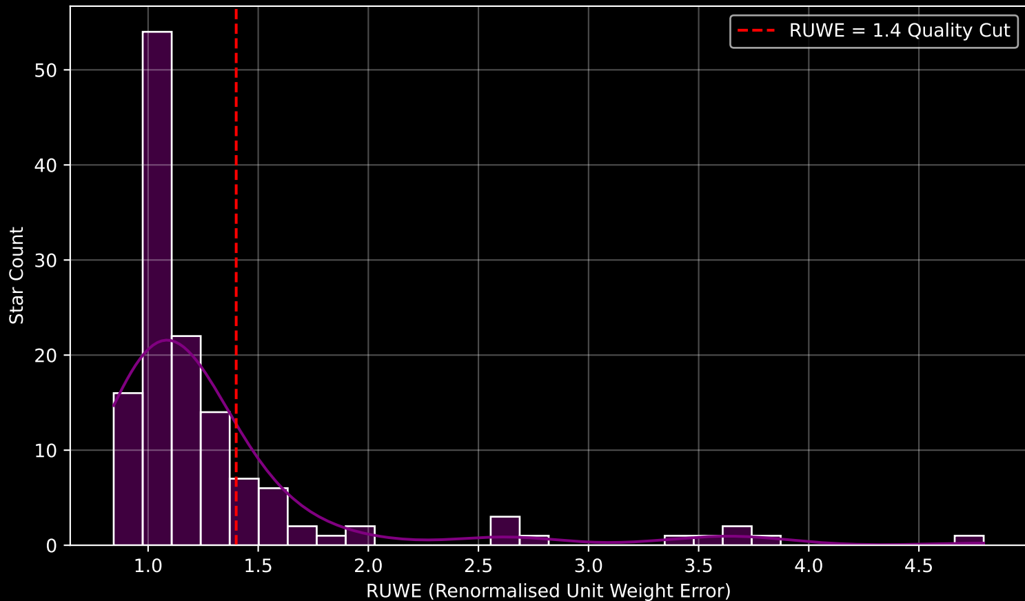
GAPOGEE DR17 Field [042+43_MGA] RUWE Distribution (n= 134)
